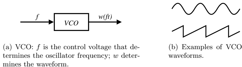
Figure 3.1: Voltage Controlled Oscillator (VCO)
