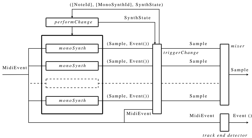
Figure 4.2: Overall structure of the polyphonic synthesizer
