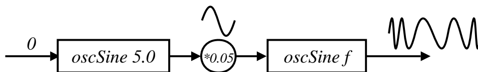
Figure 3.2: Modulating an oscillator to obtain vibrato
