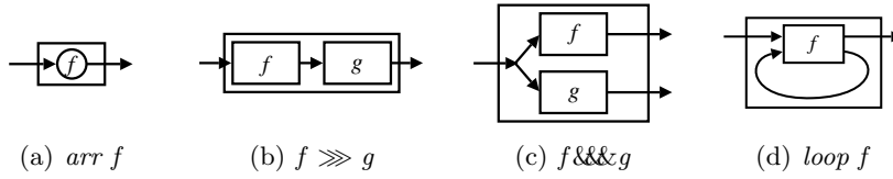
Figure 2.2: Basic signal function combinators.
