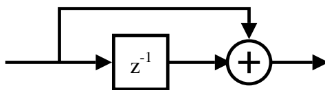
Figure 3.6: Simplest possible digital low-pass filter
