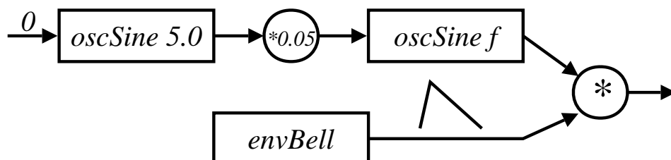
Figure 3.7: Vibrato and bell-like envelope
