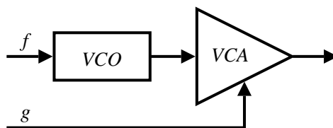
Figure 3.4: Basic synthesizer patch: f controls the frequency, g is the gate signal.
